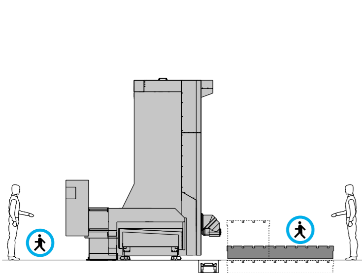
RONIN 300/400 SOLUTION RONIN 300/400 shape design - Morfologia RONIN 300/400 - Bauform der Ronin - Morphologie Ronin
